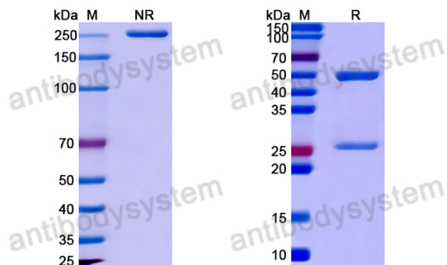
SDS PAGE for DNA Antibody (N4-10)
