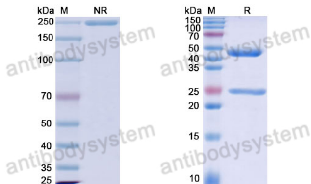
SDS PAGE for DNA Antibody (111.48)
