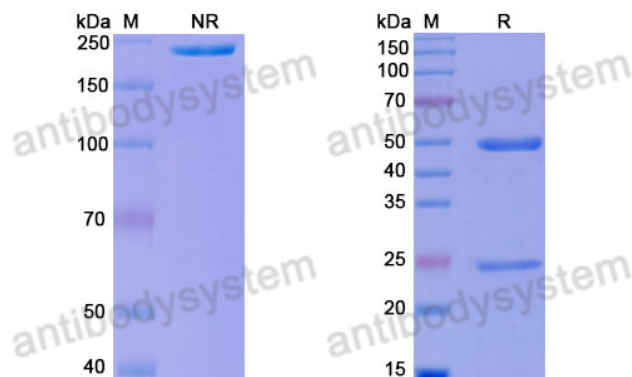
SDS PAGE for DNA Antibody (165.44)
