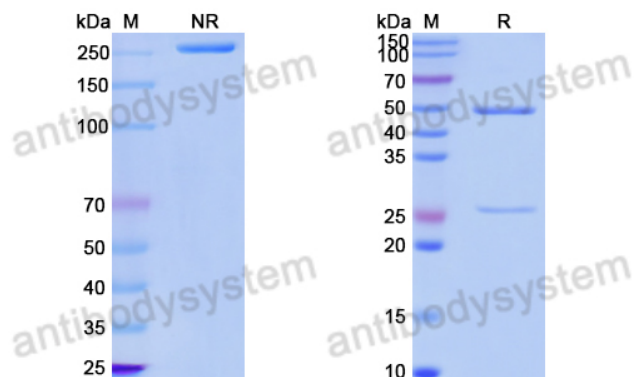
SDS PAGE for DNA Antibody (111.67)
