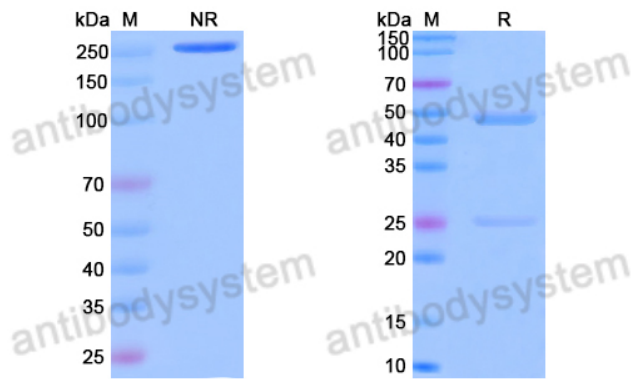
SDS PAGE for DNA Antibody (111.19)
