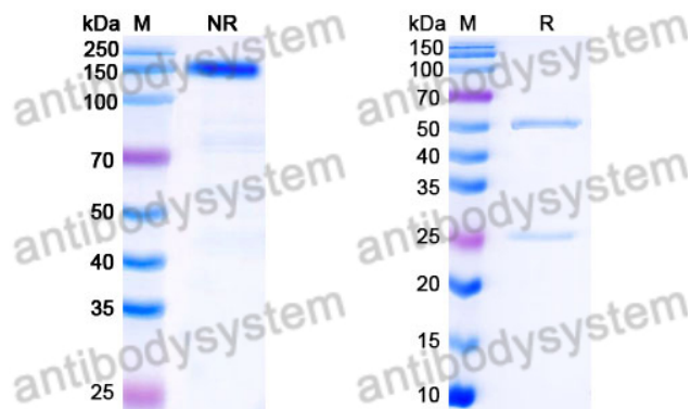
SDS PAGE for Rat IgG1, kappa Isotype Control Antibody (RTK2071)
