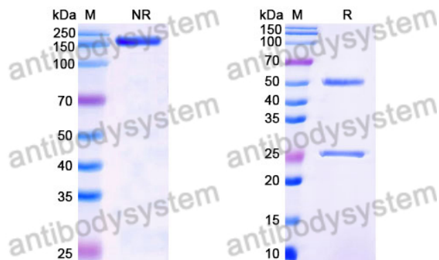
SDS PAGE for Mouse IgG3, kappa Isotype Control Antibody (J606)
