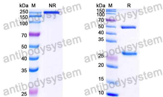
SDS PAGE for Mouse IgG2a Isotype Control Antibody (GC270)
