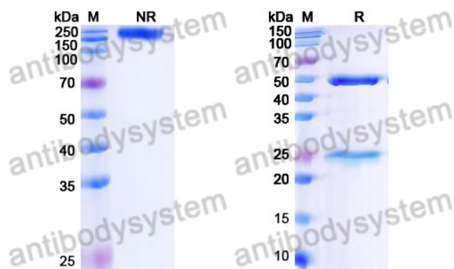
SDS PAGE for Human IgG1 (LALAPG) Isotype Control Antibody (HyHEL-10)
