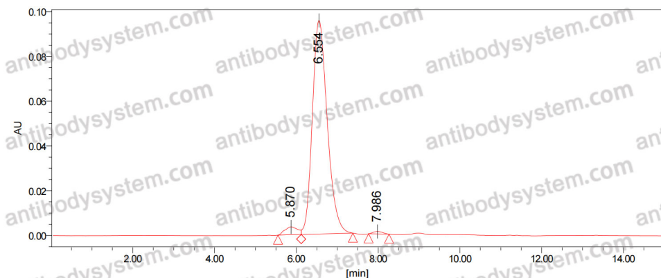
SEC-HPLC
