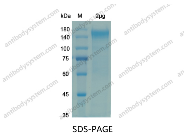
SDS PAGE for recombinant SARS-CoV-2 S1 Protein
