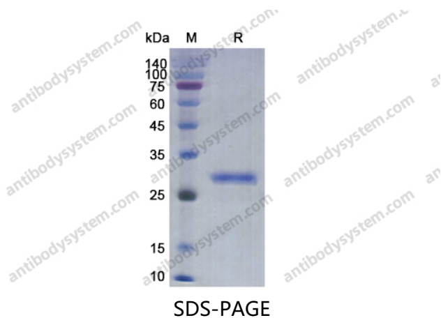
SDS PAGE for recombinant Human IL34
