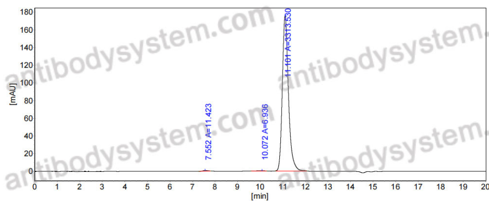
SEC-HPLC
