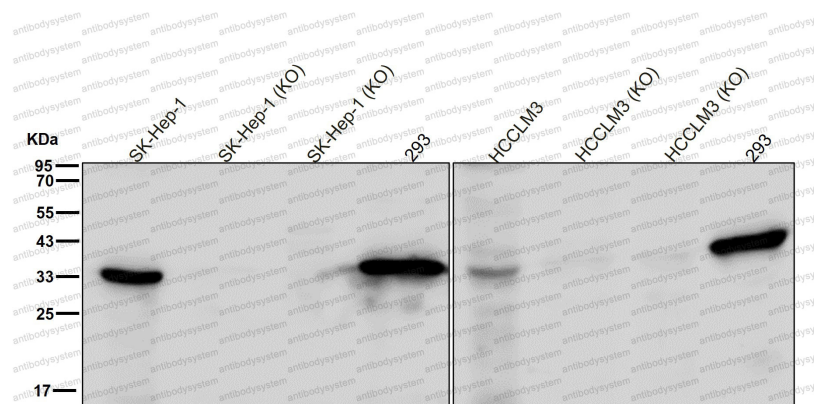
Western blot
