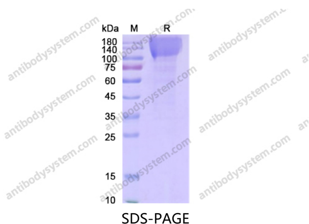
SDS PAGE for recombinant Human CD66e / CEA / CEACAM5
