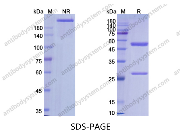
SDS PAGE for Lemalesomab
