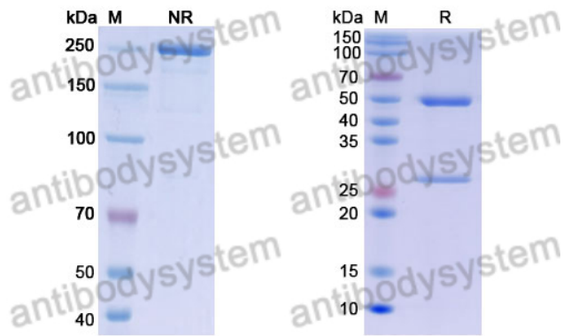
SDS PAGE for DENV-4 Envelope protein E/EDIII domain Antibody
