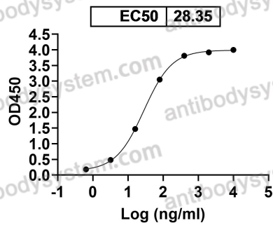
Anti-Human CD40/TNFRSF5 Antibody (Iv0136) binds with CD40
