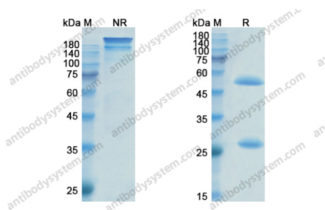
SDS PAGE for Pinatuzumab
