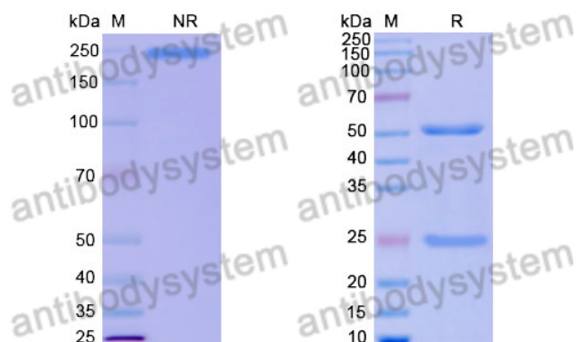
SDS PAGE for Human IgG4 (S228P), Lambda Isotype Control Antibody (HyHEL-10)
