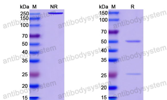
SDS PAGE for HIV-1 gp140/Env Trimer Broadly Neutralizing Antib
